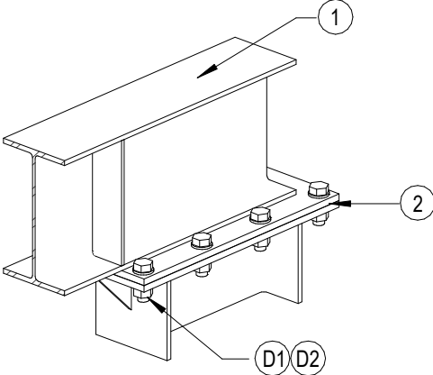
HEADER WELDMENTS TO COLUMN WELDMENTS DETAIL "D"
