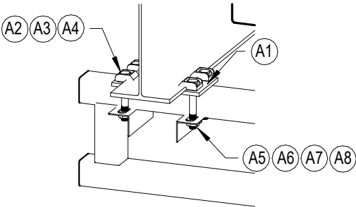
TRACK TO HEADER WELDMENTS DETAIL "A"
