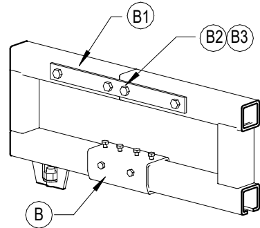
TRACK SPLICE TO TRACK SECTIONS DETAIL "B"
