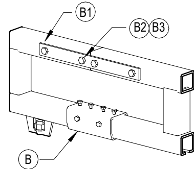
TRACK SPLICE TO TRACK SECTIONS
