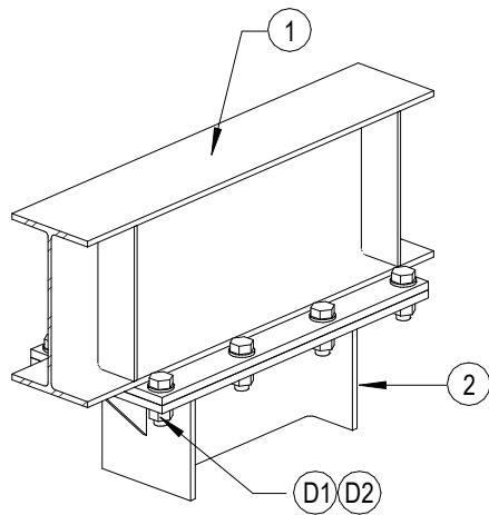
HEADER WELDMENTS TO COLUMN WELDMENTS
