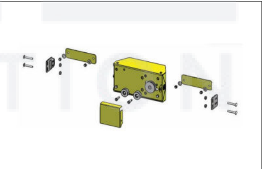
⑧ ELECTRICAL KIT
