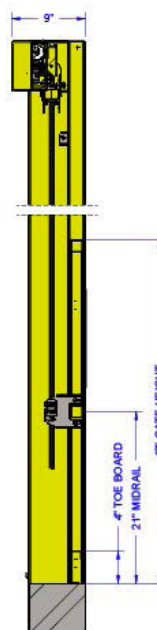
SIDE VIEW "GATE CLOSED"
