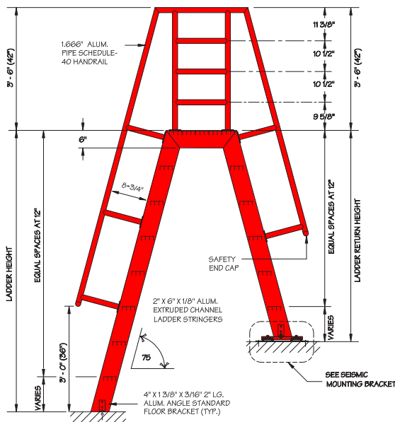
Ship Ladder with Access to Roof Hatch
