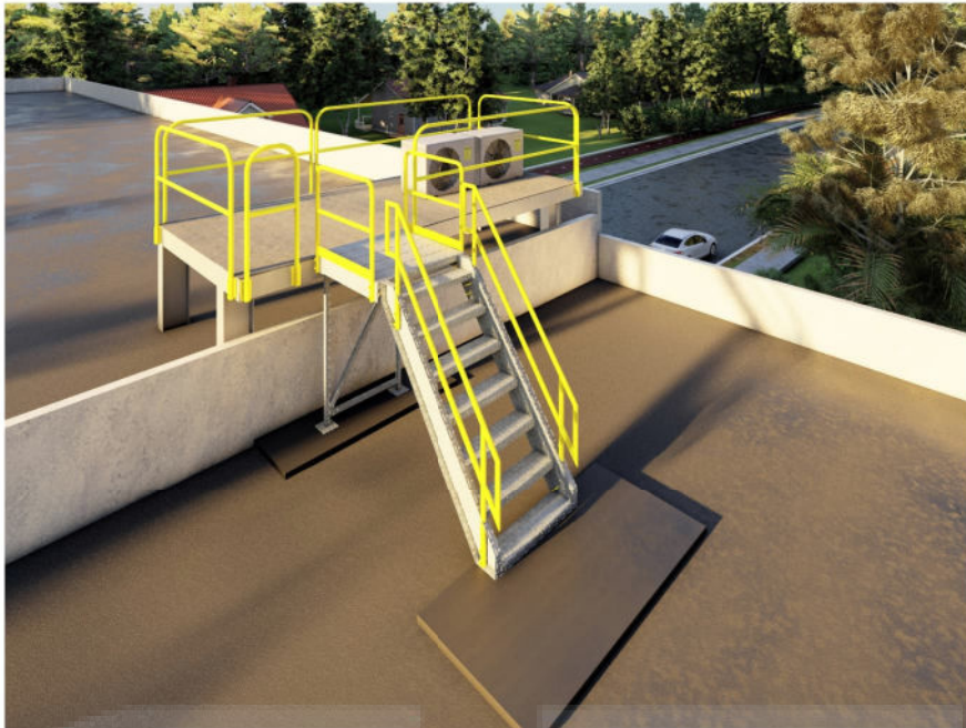
ROOF ACCESS STAIR WITH PLATFORM LANDING
