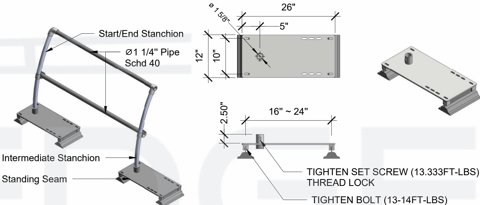
AccuFIT with Standing Seam
