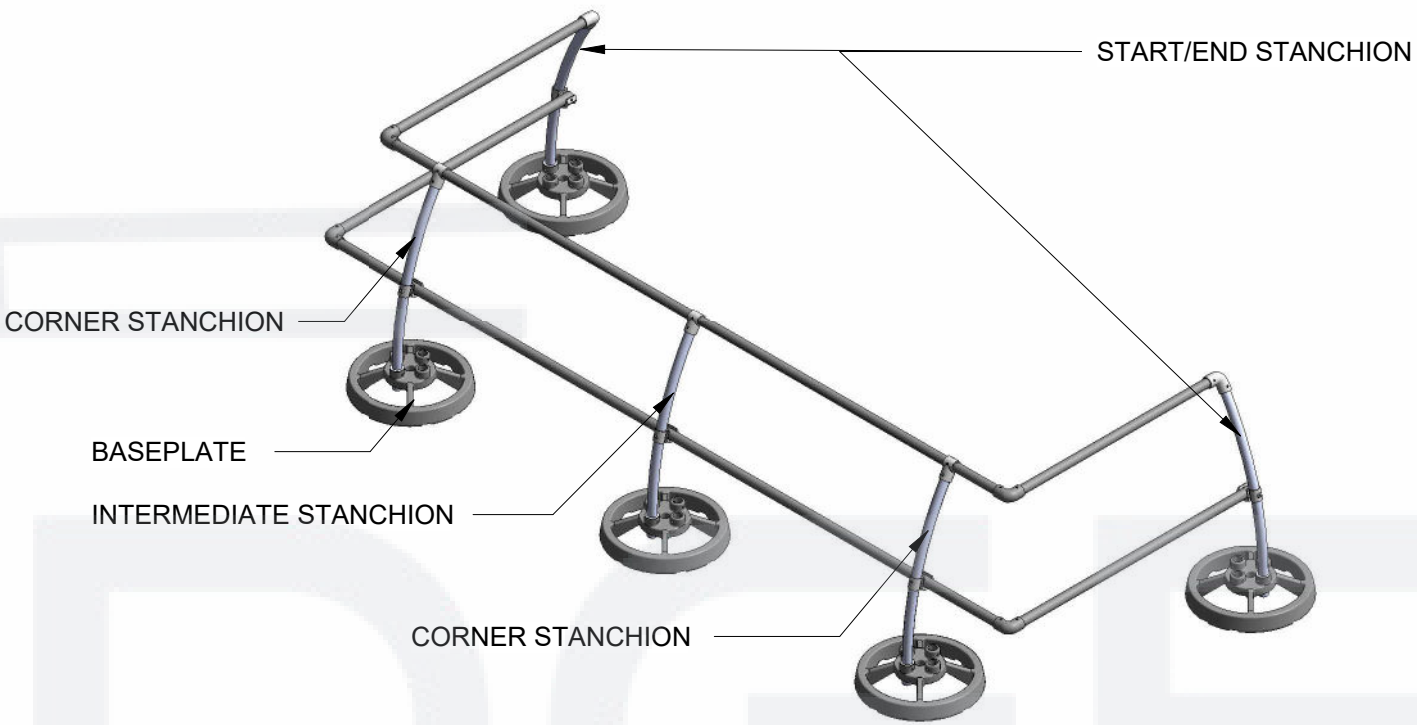
ACCUFIT (CURVED STANCHION) ROOF RAILING ASSEMBLY
