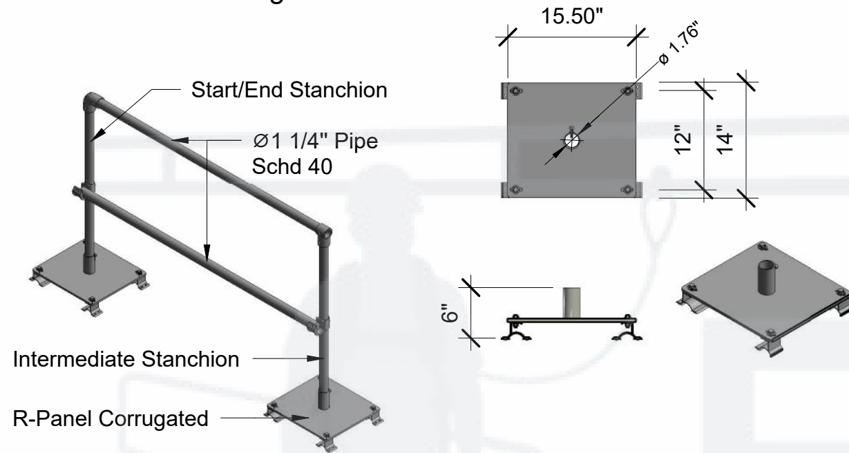
AccuFIT with Corrugated
