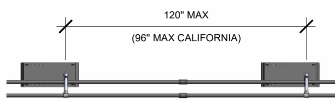
DETAIL B PERPENDICULAR TO SEAM
