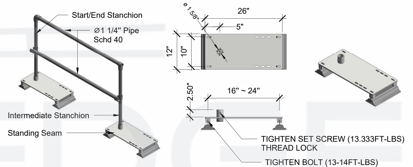
AccuFIT with Standing Seam
