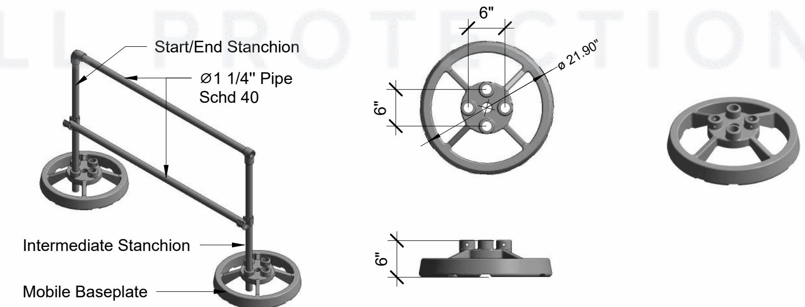
AccuFIT with Mobile Baseplate
