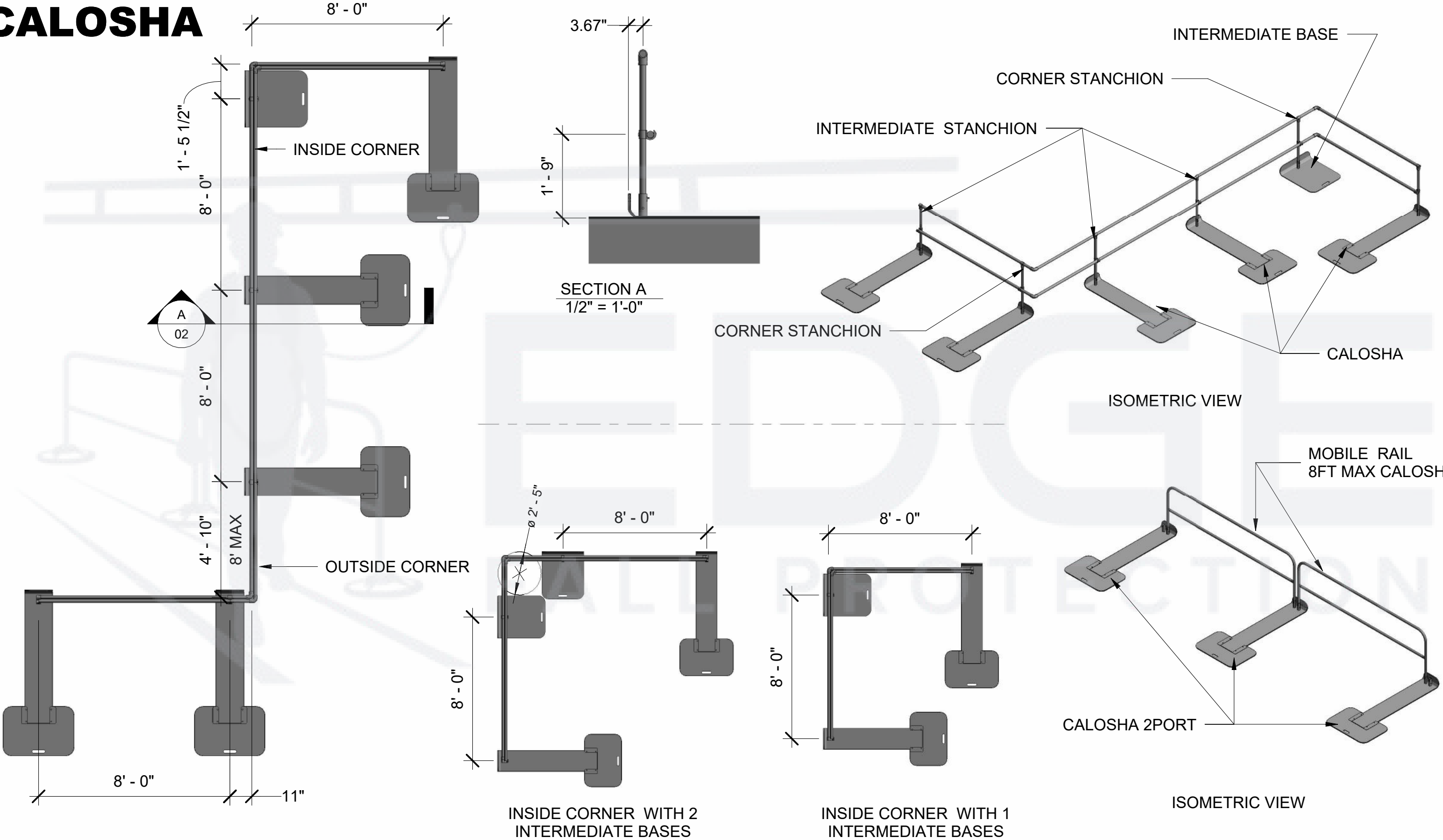
CORNER ASSEMBLY DETAIL
