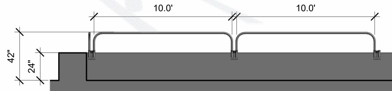
DETAIL A
