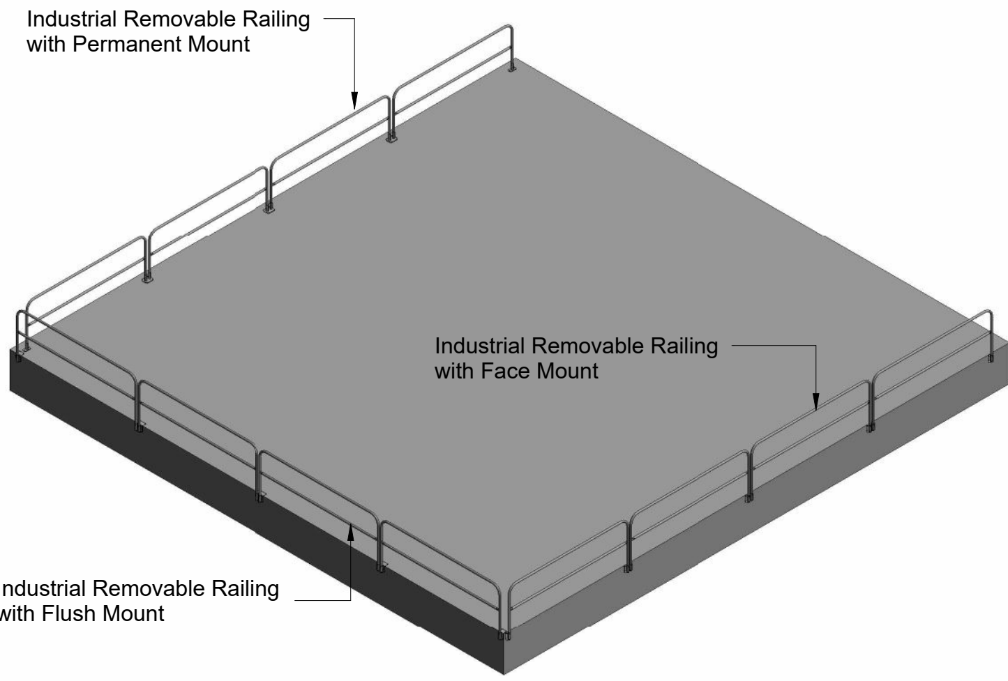
ISOMETRIC VIEW
