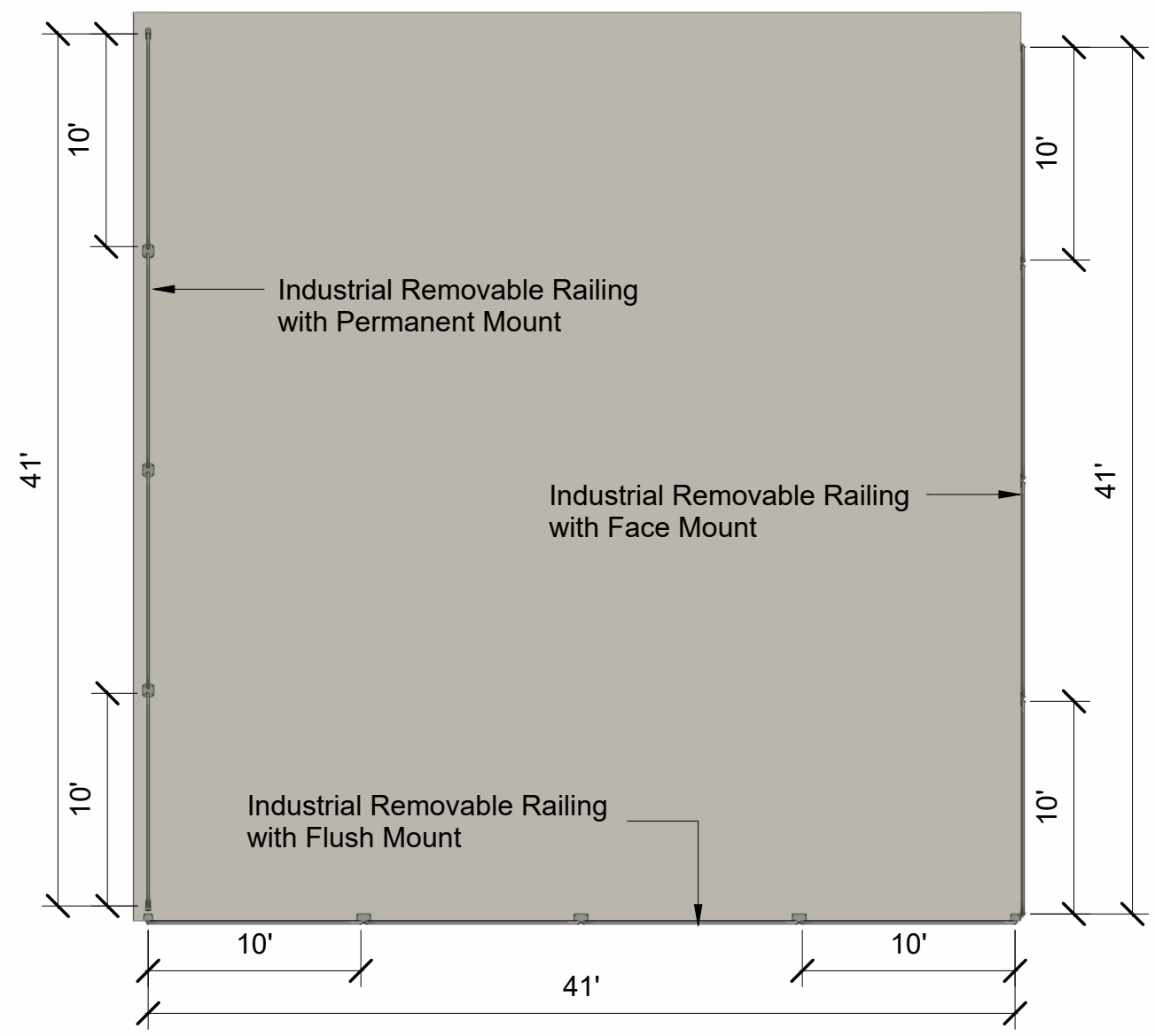
PLAN LAYOUT
