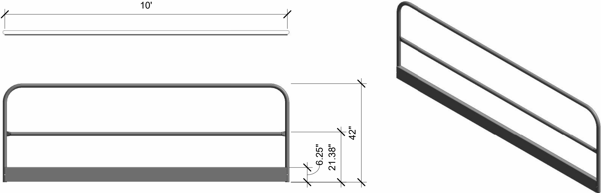
"10FT" Floor Mounted Construction Rail with Toeboard
