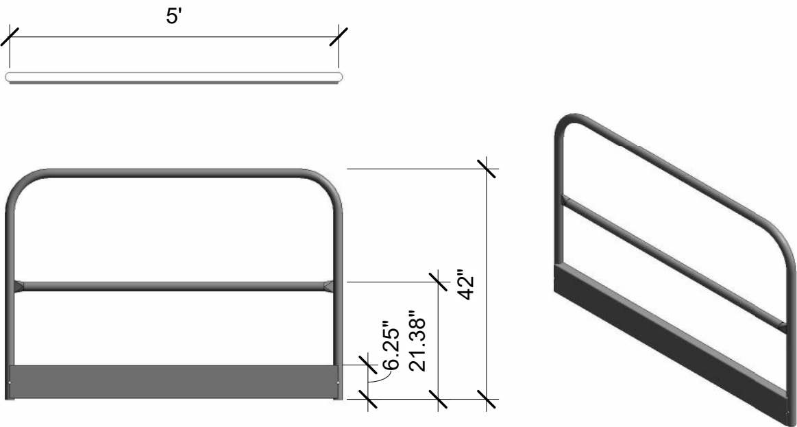
"5FT" Floor Mounted Construction Rail with Toeboard
