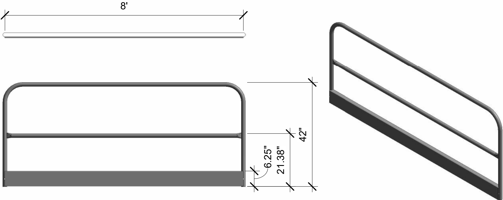
"8FT" Floor Mounted Construction Rail with Toeboard
