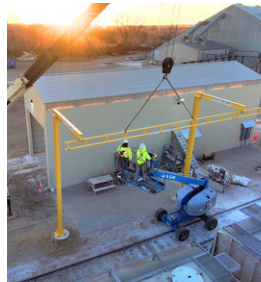
Exterior Fall Arrest
